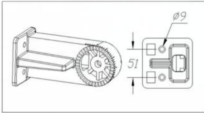
B2 Bracket
